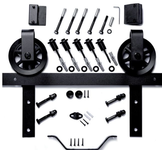
Montageset Assembly set # 106207200
